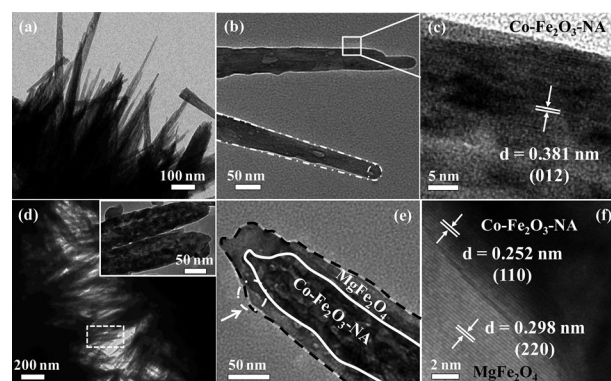
Figure 2. TEM and HRTEM images of the Co-Fe 2 O 3 -NA (a–c) and Co-Fe 2 O 3 -NA/MgFe 2 O 4 heterojunction (d–f).
